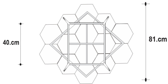
BaseView
