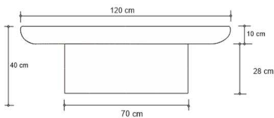
Base View
